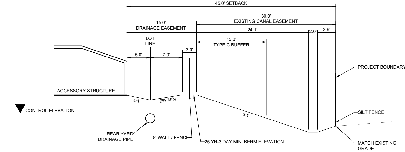
SECTION B-B EAST ABUTTING DRAINAGE CONVEYANCE ADJACENT TO STATE PRESERVE SECTION NTS
