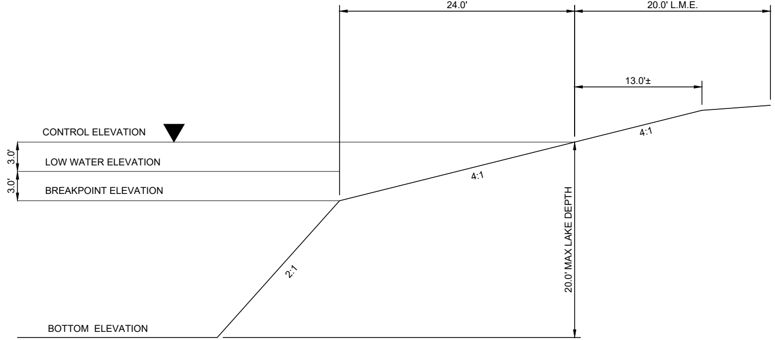
PROPOSED TYPICAL LAKE CROSS SECTION NTS
