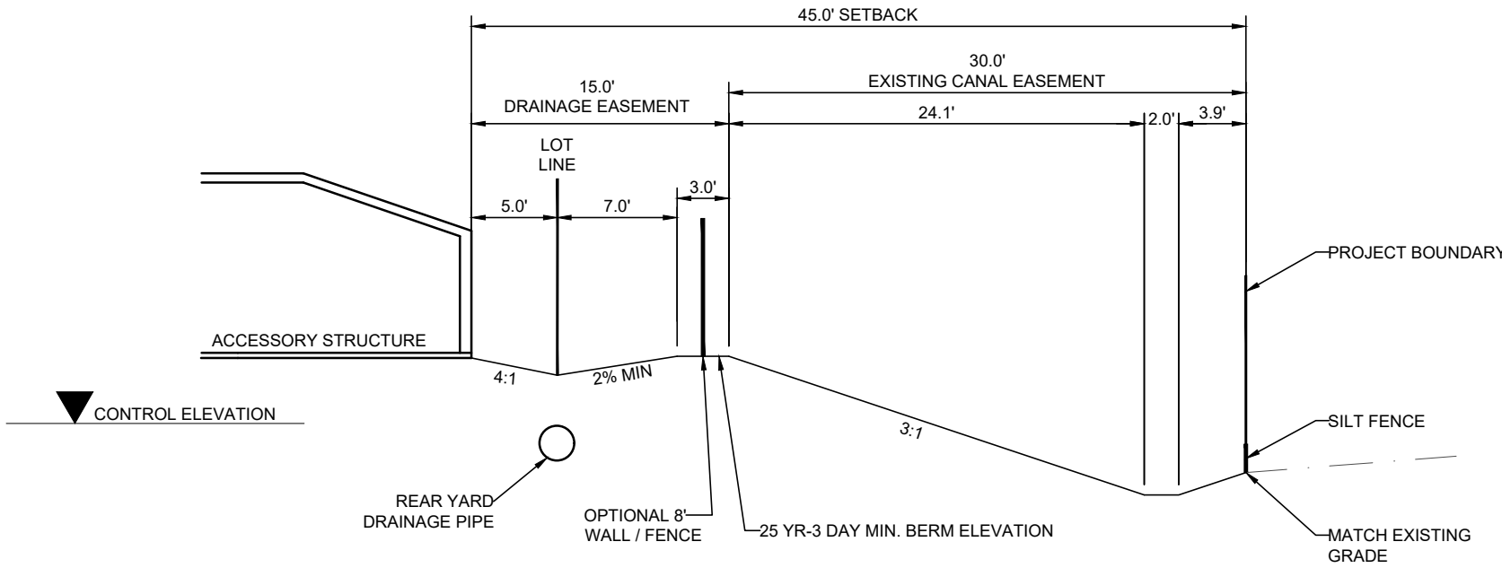
SECTION A-A EAST ABUTTING DRAINAGE CONVEYANCE SECTION NTS
