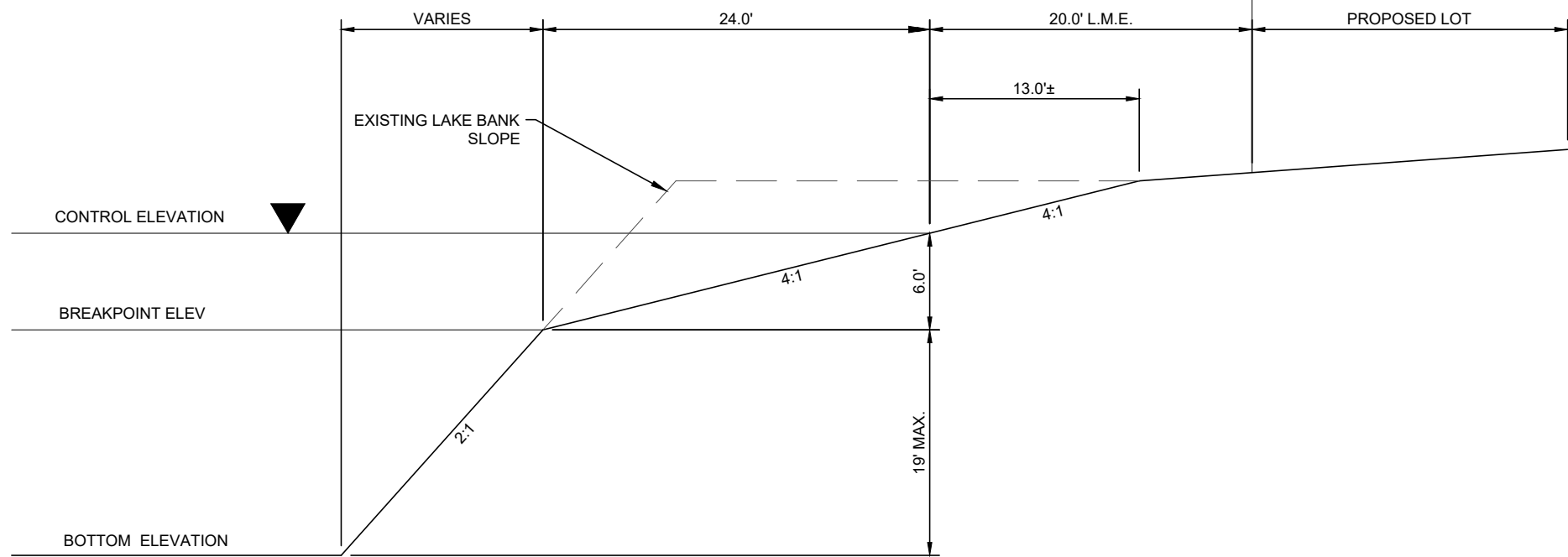
TYPICAL RECLAIMED LAKE SECTION NTS
