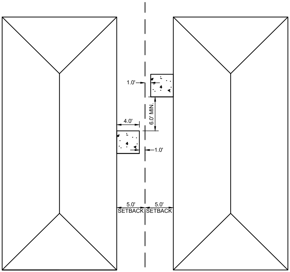
PLAN VIEW
