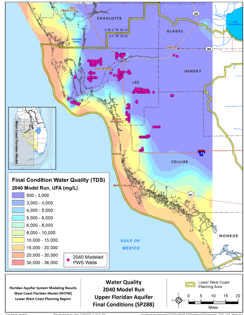
Figure D-27. Upper Floridan aquifer water quality (total dissolved solids concentrations) for the final condition of the 2040 model run.
