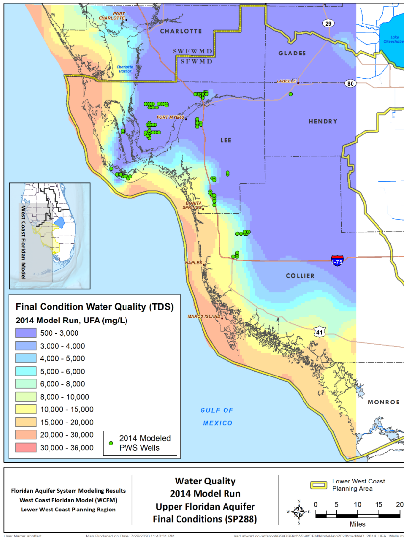
Figure D-26. Upper Floridan aquifer water quality (total dissolved solids concentrations) for the final condition of the 2014 model run.
