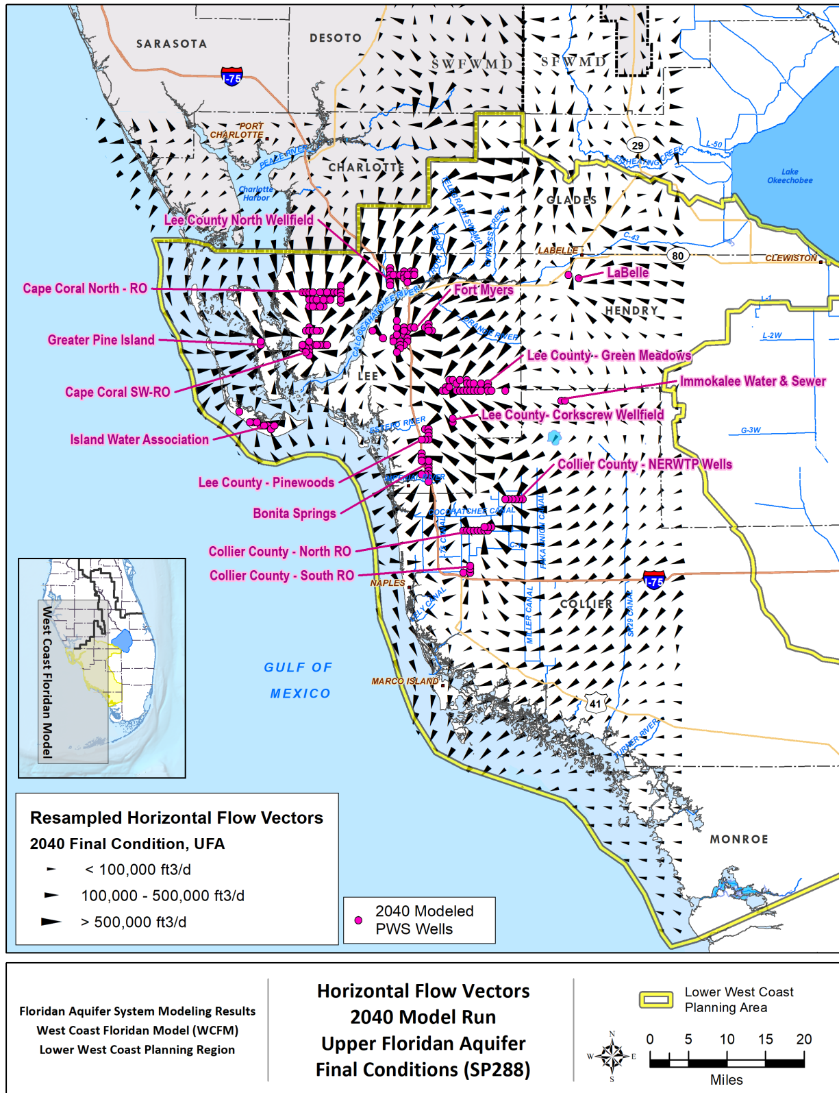
Figure D-33. Resampled horizontal flow vectors for the final condition of the 2040 model simulation in the Upper Floridan aquifer.
