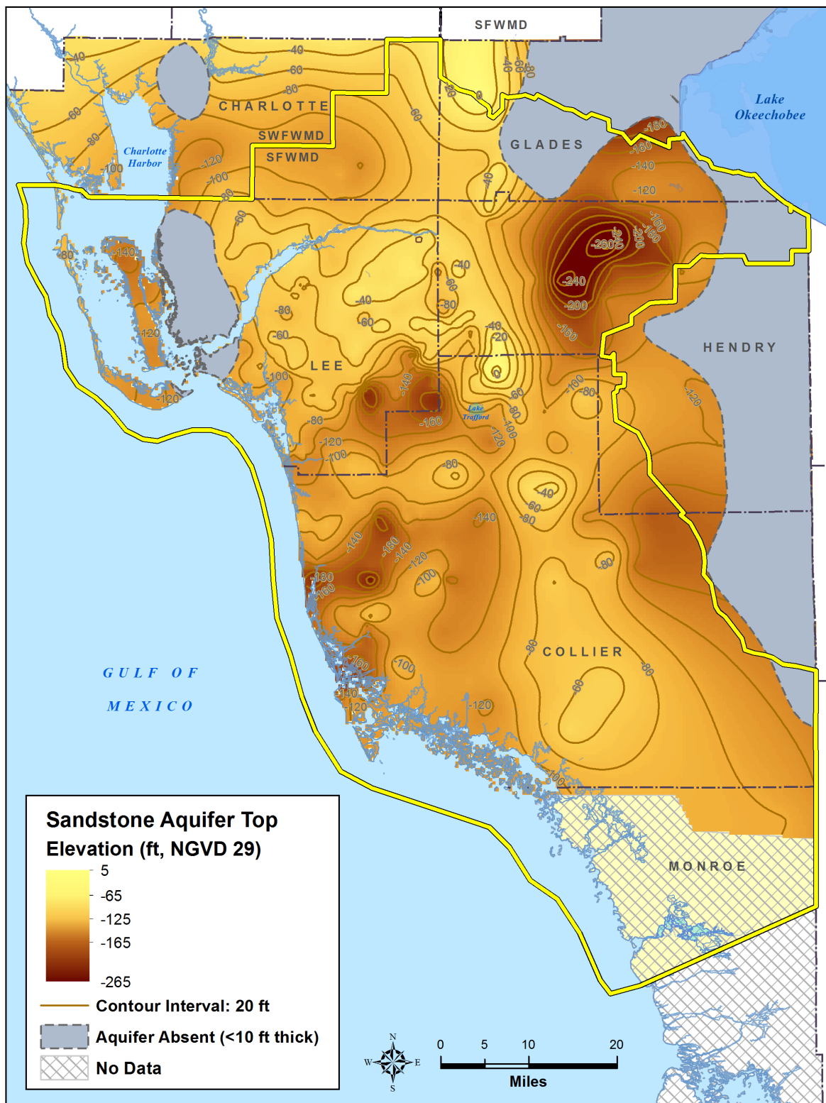
Figure C-7. Structural top (MFL) of the Sandstone aquifer in the LWC Planning Area.
