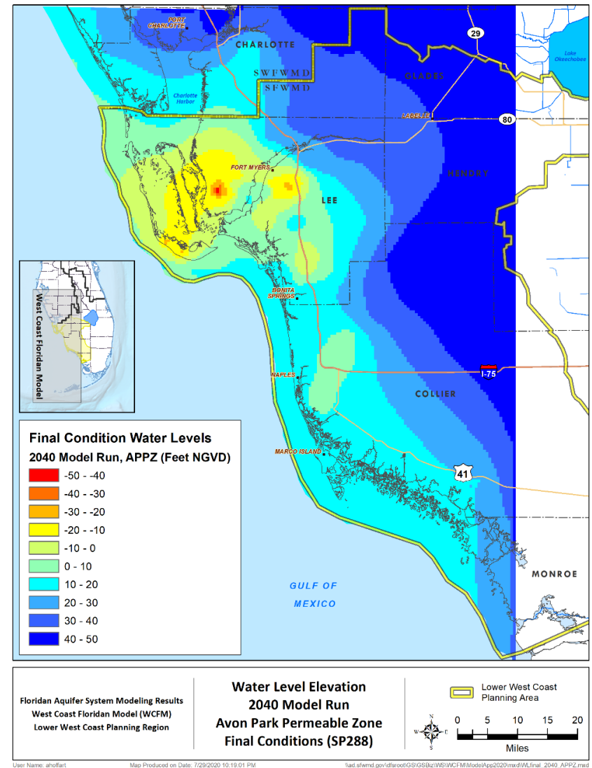
Figure D-24. Avon Park permeable zone water levels for the final condition of the 2040 model run.
