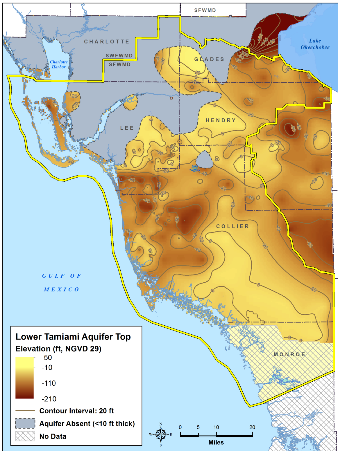
Figure C-6. Structural top (MFL) of the Lower Tamiami aquifer in the LWC Planning Area.
