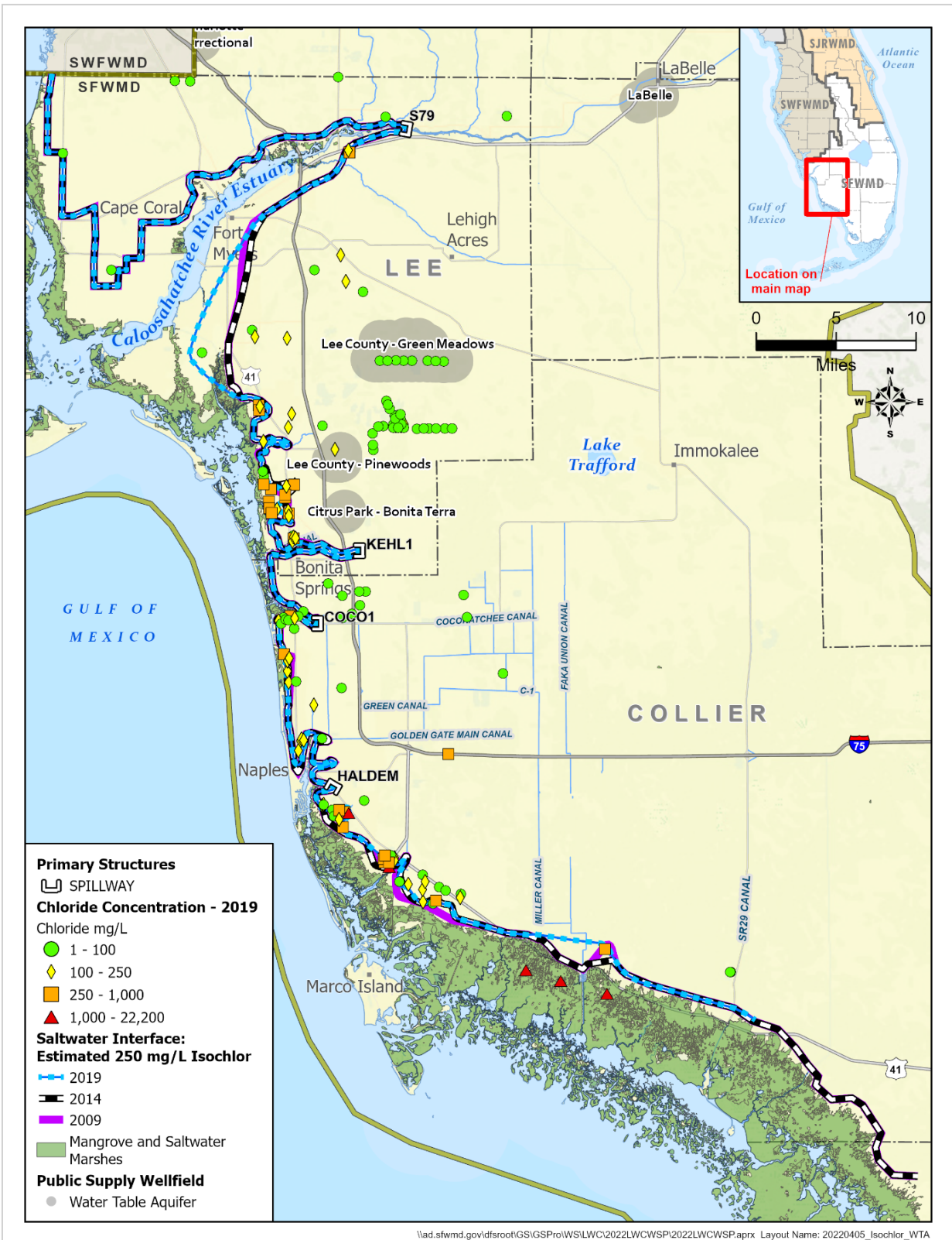
Figure D-1. Estimated position of the saltwater interface in 2009, 2014, and 2019 in the Water Table aquifer in Lee and Collier counties.
