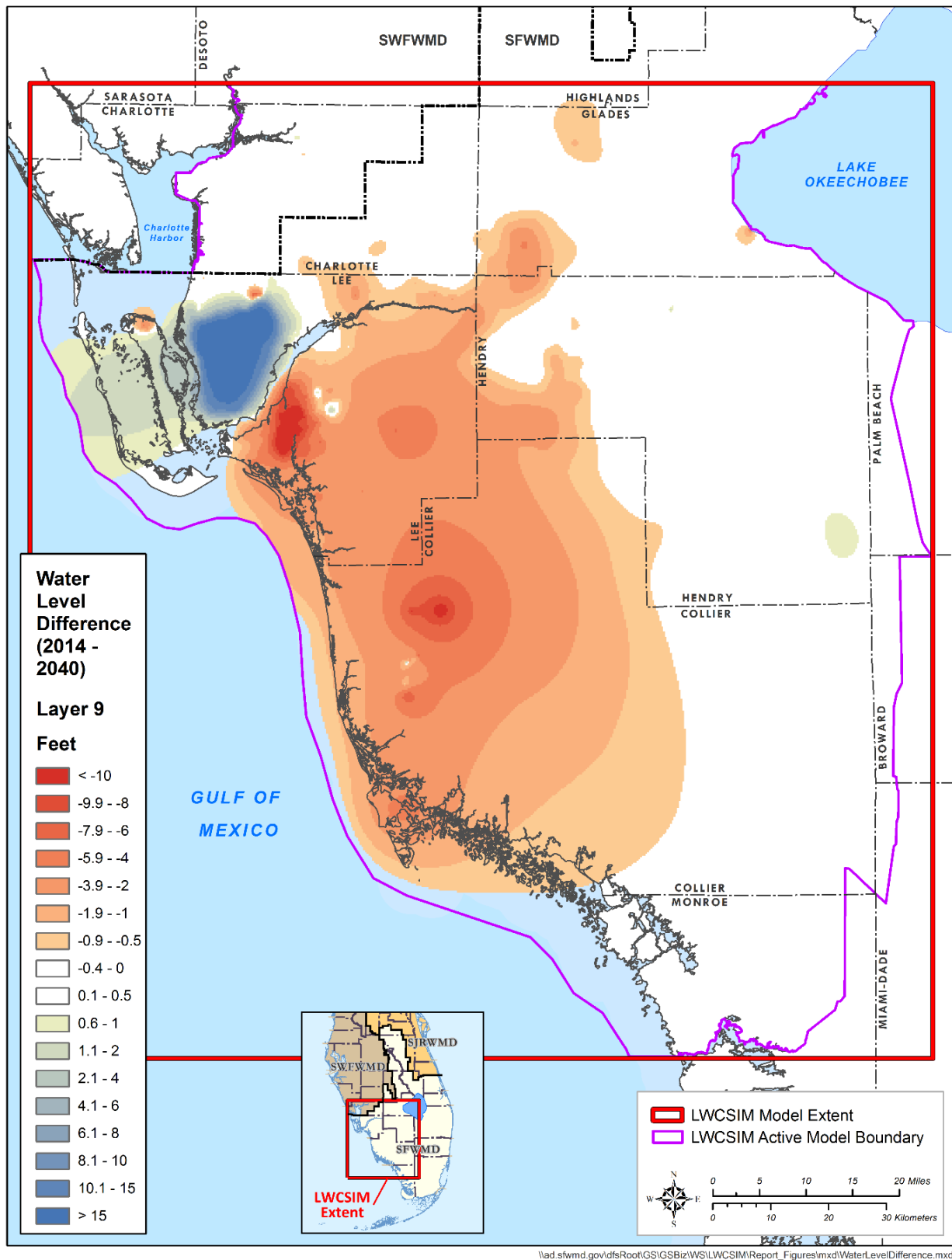
Figure D-11. 2014 to 2040 water level difference in the Mid-Hawthorn aquifer.
