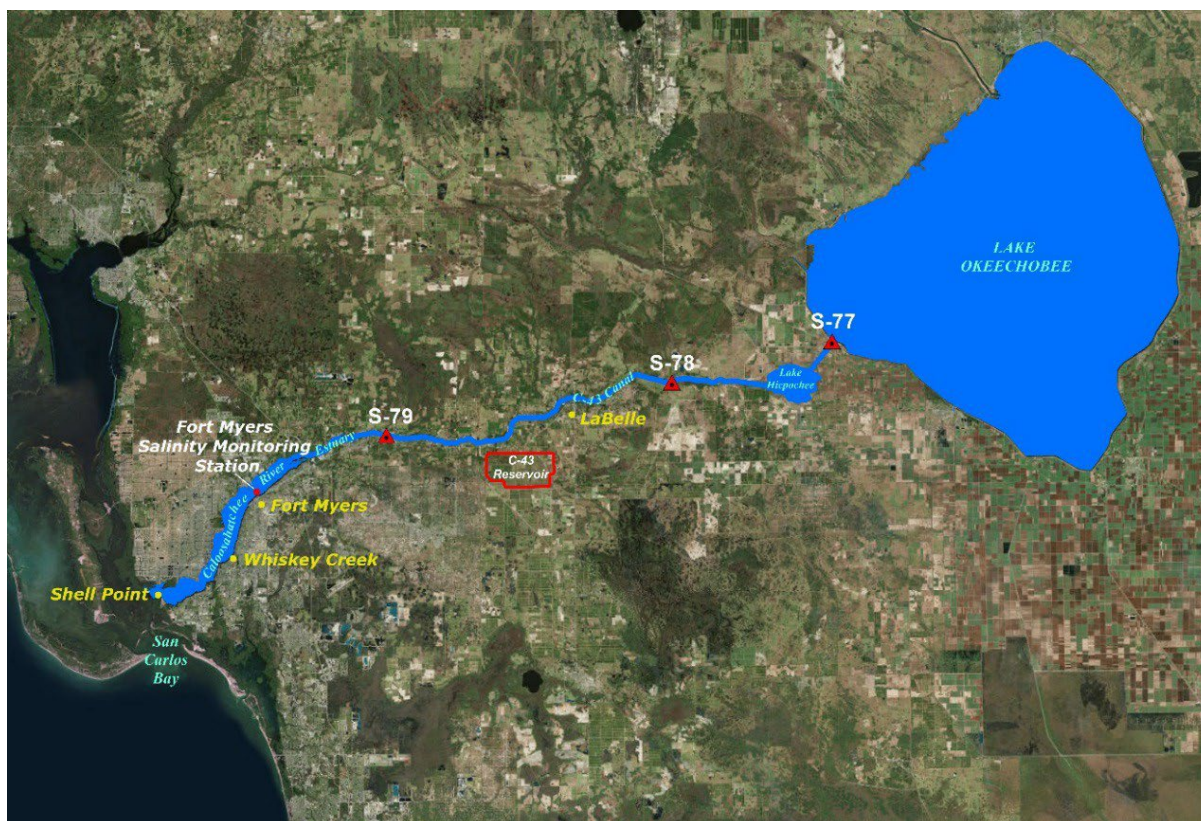
Figure C-2. Caloosahatchee River minimum flow and minimum water level waterbody (downstream of S-79), showing the hydrologic connection to Lake Okeechobee.
