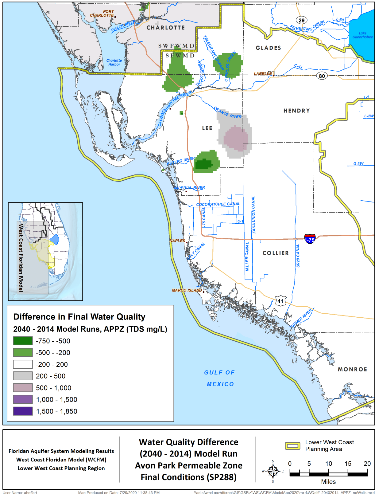
Figure D-31. Avon Park permeable zone water quality (total dissolved solids concentration) difference between 2014 and 2040.
