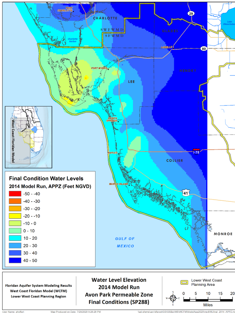
Figure D-23. Avon Park permeable zone water levels for the final condition of the 2014 model run.
