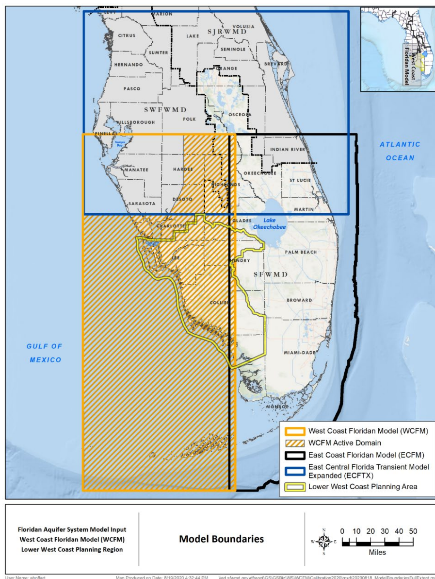
Figure D-18. Model boundaries of three Floridan aquifer system regional groundwater models in Central and South Florida.
