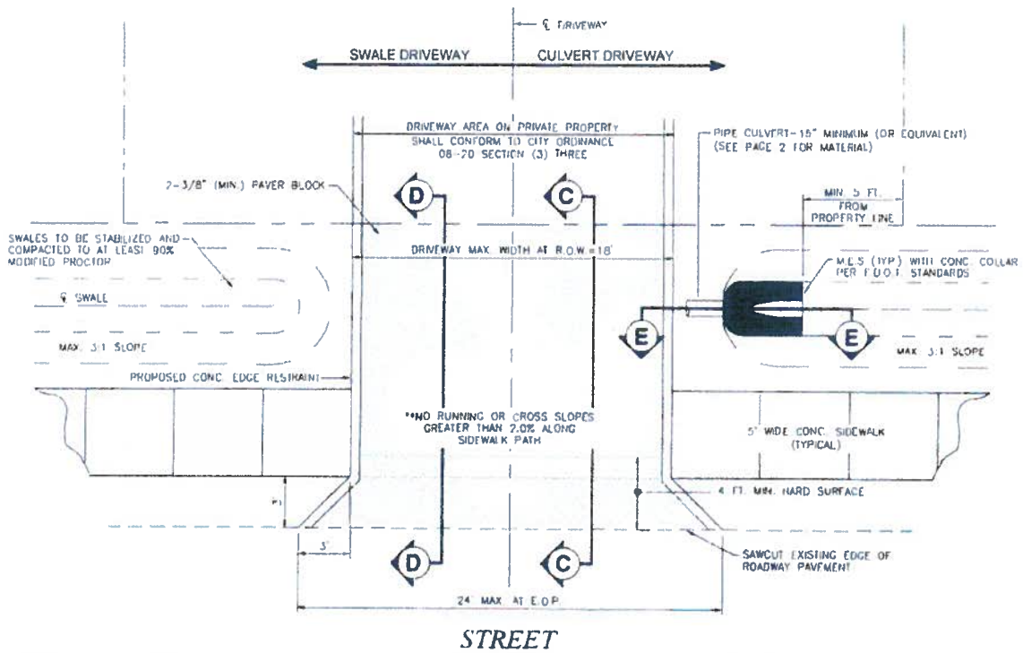
FIGURE 2A PAVER BLOCK RESIDENTIAL DRIVEWAY
